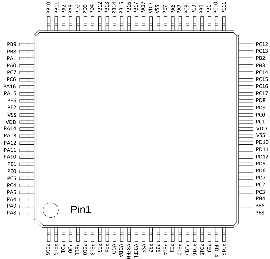
Figure 9-2 LQFP100 package
