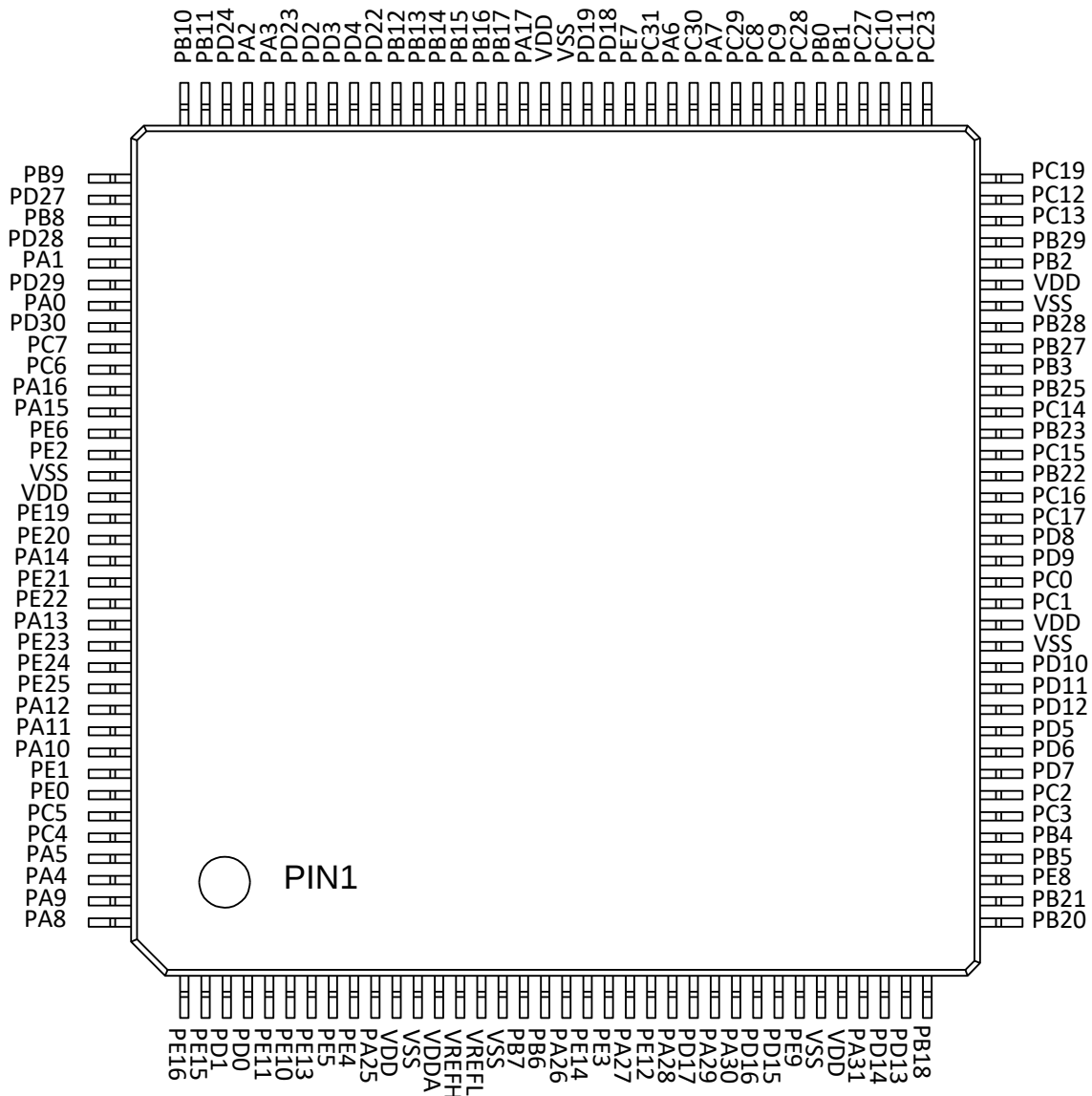
Figure 9-1 LQFP144 package
