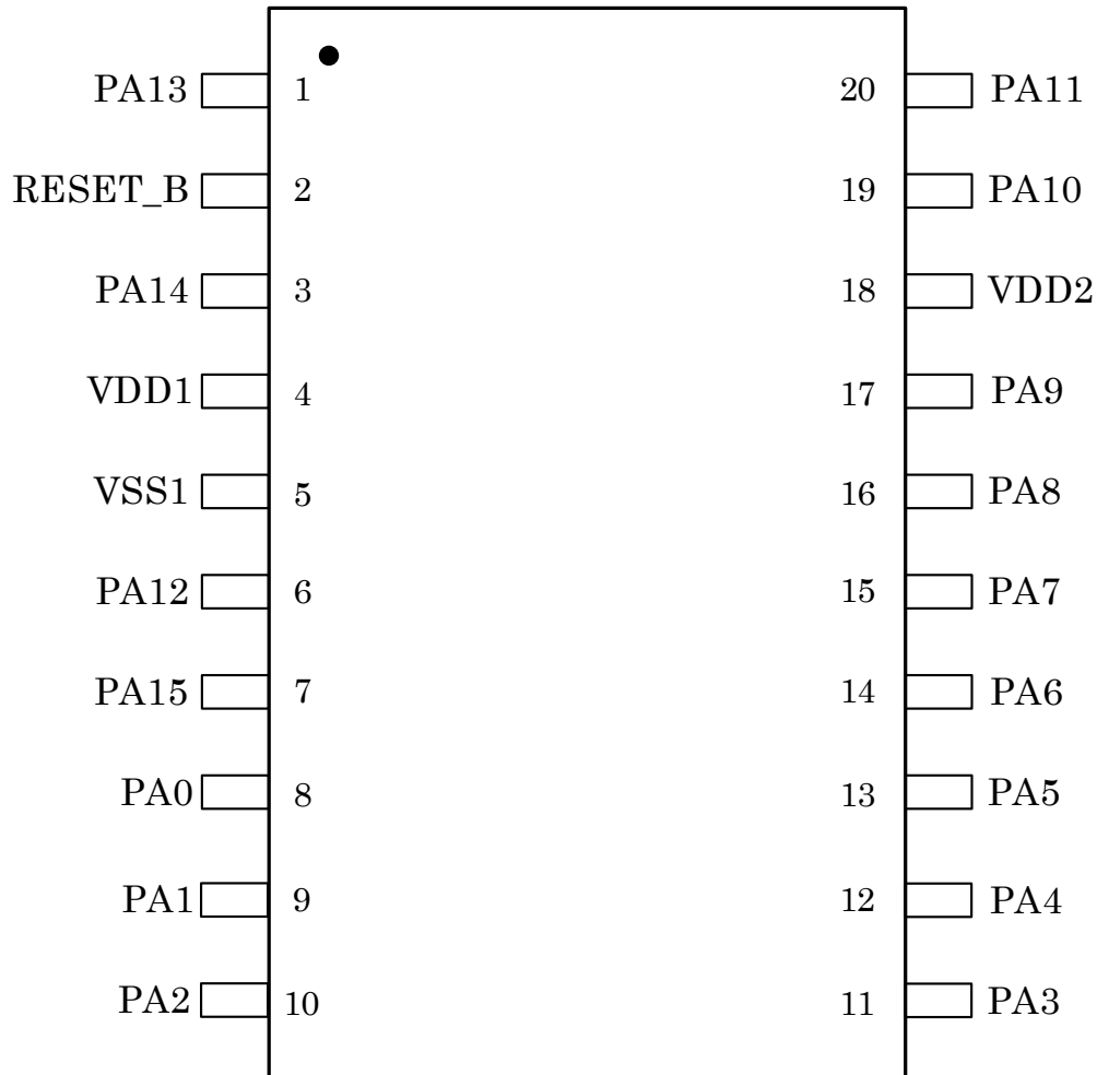
Figure 9-3 20-pin TSSOP20 package
